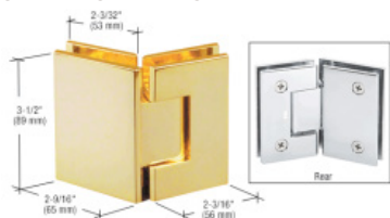
135 Degrees glass to glass hinge
